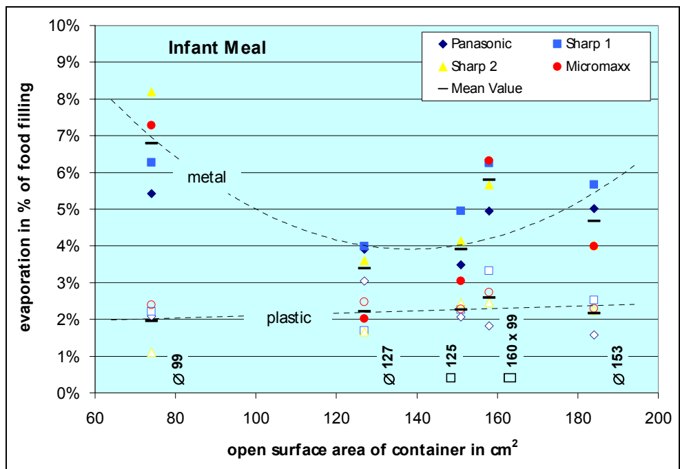
Figure 6.12: Water evaporated from infant meal during microwave heating in percent of mass of food filling.
