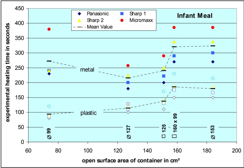
Figure 6.9: Used heating times in microwave heating experiments with containers filled with infant meal. The heating times were adjusted to achieve an average temperature increase from 10°C to 75°C.
