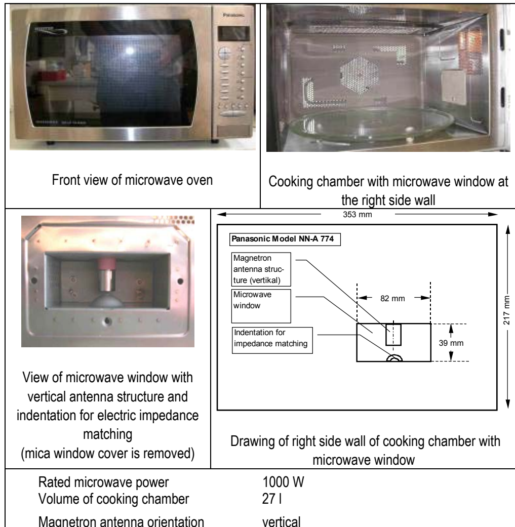
Figure B.1: Panasonic Microwave Oven Model NN-A764 - Inverter oven (Panasonic)
