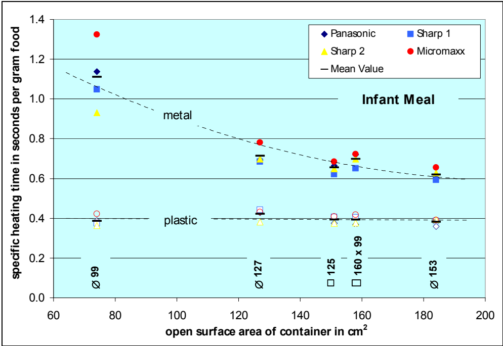
Figure 6.10: Specific heating time seconds per gram product and normalised to a 1000 W oven. Values calculated from real heating times in figure 6.9.
